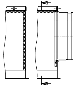
internal (-Ii)
